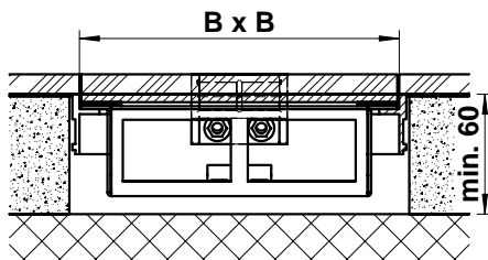
Detail o
