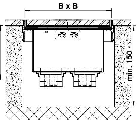
Detail m 2
