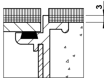
Detail m
