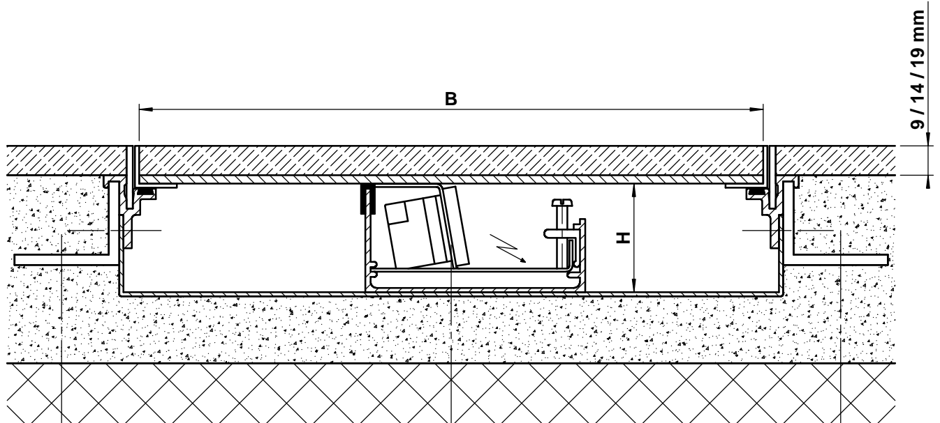
Detail m 2
