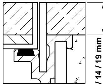
Detail m 2
