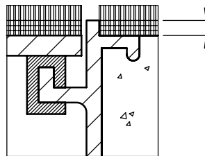
Detail m
