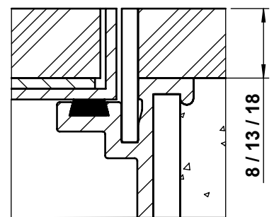
Detail m 2
