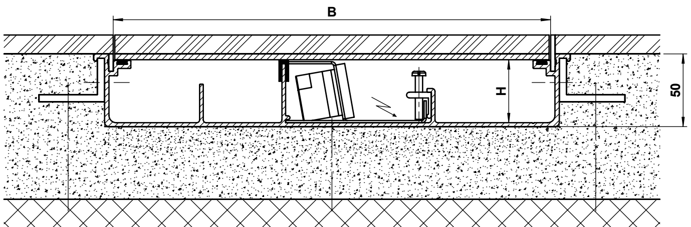
Detail o
