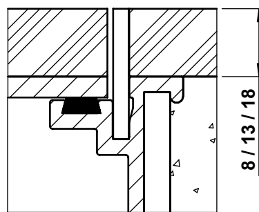
Detail m
