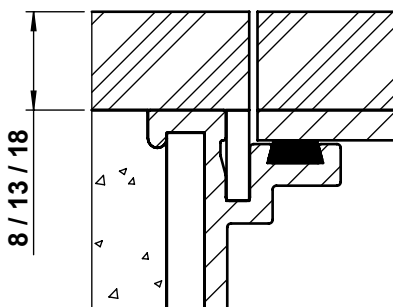
Detail o
